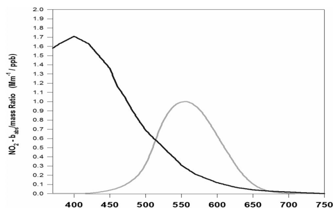
Figure 2. NO 2 absorption coefficient and 2° observer PR curves as a function of wavelength ( \eta m ).
